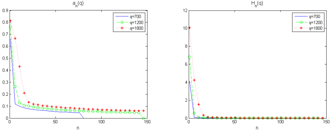
Figure 3: The acceptance rate (left panel) and the hiring rate (right panel).
