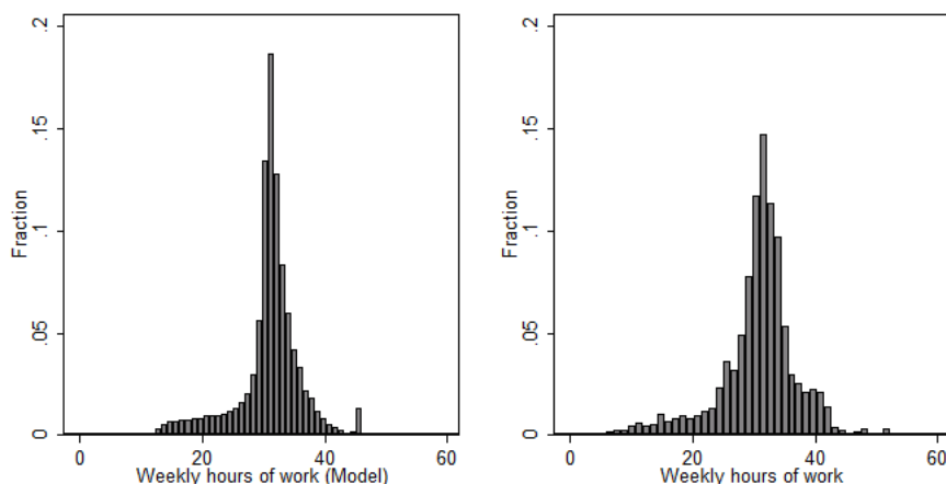
Figure 5: Hours distribution in the model (left panel) and data (right panel).
