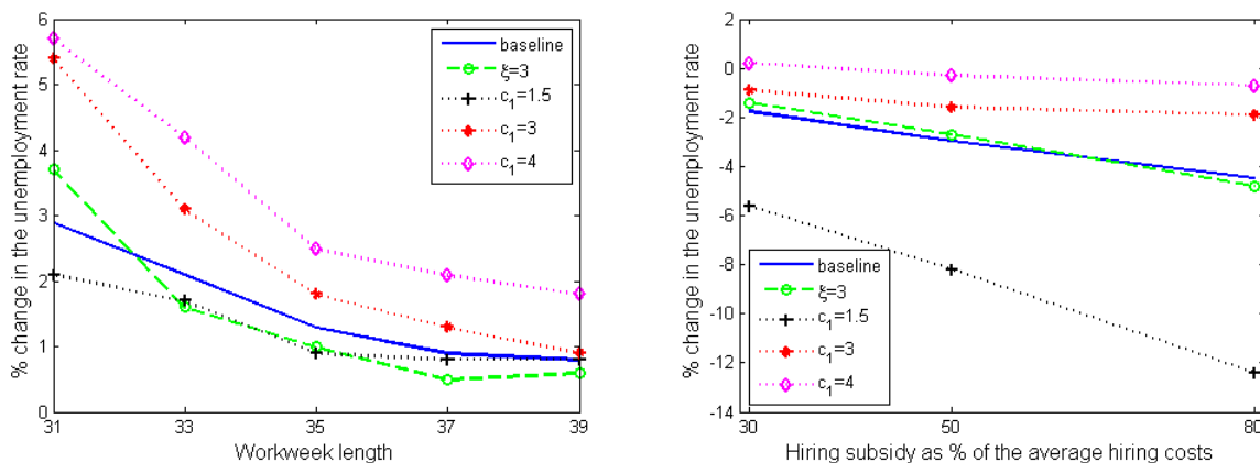
Figure 6: Robustness check
