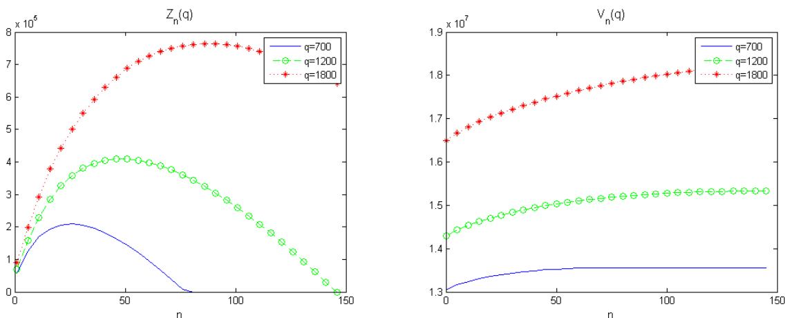
Figure 2: The value added of a match (left panel) and the value of a firm (right panel).
