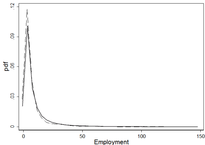
Figure 4: Size distribution in the data (solid line) and in the model (dashed line)
