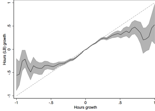
Figure 8: The relationship between the growth rates of actual and lower bound work hours.
